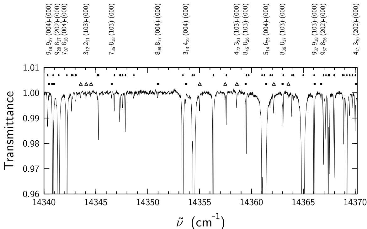
FIG. 5. Sample spectrum plus new line assignments. The small diamonds at the top of the spectrum denote previously assigned lines; newly assigned lines have assignments above the figure and are marked in the spectrum with filled circles for \text{H}_2^{16}\text{O} lines and open triangles for \text{H}_2^{18}\text{O} lines.
